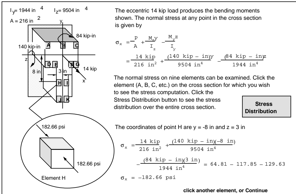
Figure 2 Computation of stresses at point H
